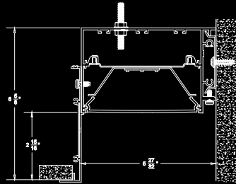
DRY WALL OVERLAP FLANGE
