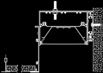
GRID FLUSH TILE
