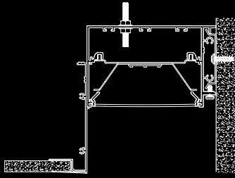
DRY WALL SPACKLE FLANGE 1/2"
