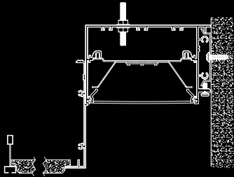
GRID SCREW SLOT TILE
