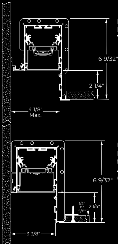
DETAIL 9/16" T-Bar Tegular Tile
