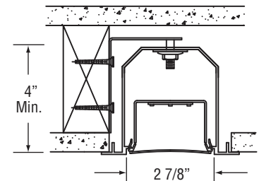
MLR3-HO-VOF Vertical Drywall Overlap Flange
