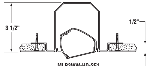
MLR3WW-HO-SF1 MLR3WW-MO-SF1 Drywall Spackle Flange
