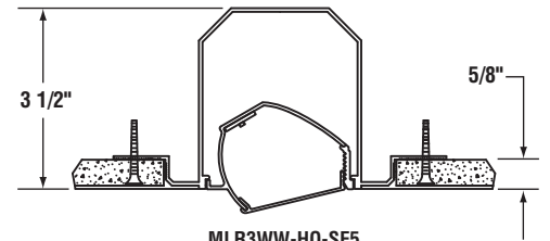
MLR3WW-HO-SF5 MLR3WW-MO-SF5 Drywall Spackle Flange
