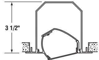
MLR3WW-HO-OF MLR3WW-MO-OF Drywall Overlap Flange
