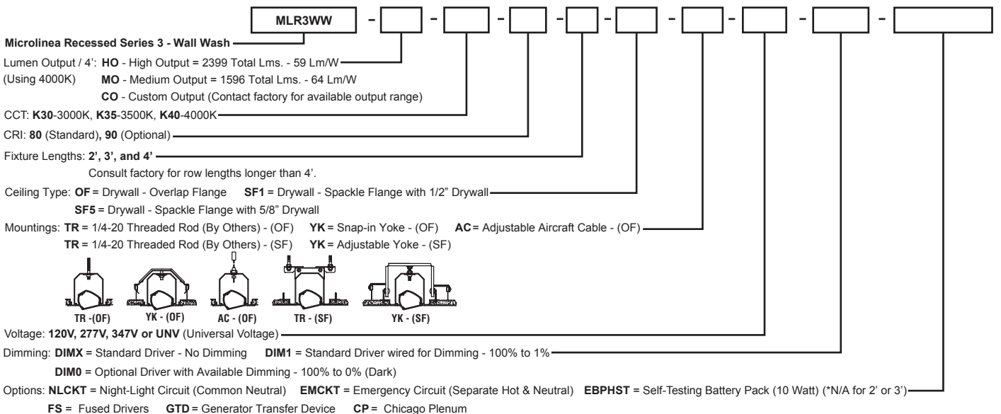
MLR3WW-HO-SF5 MLR3WW-MO-SF5 Drywall Spackle Flange
