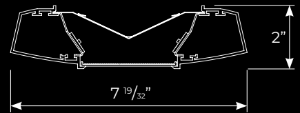
CURVED SUSPENDED
