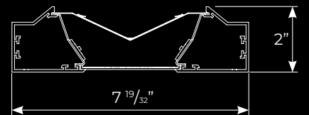
RECTANGULAR SUSPENDED
