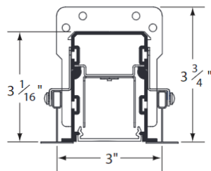
MLR2 - GRID CEILING FLUSH TILE, REGULAR TILE & SCREW SLOT
