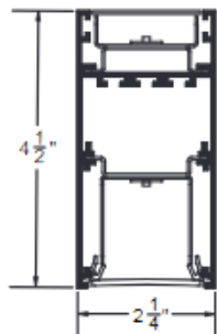
MLS2-I/D-HO/HO-FDC/LOH MLS2-I/D-MO/MO-FDC/LOH Shown with optional Frosted Dust Cover
