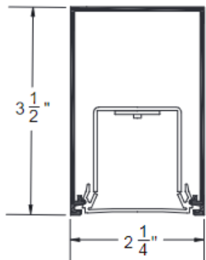
MLS2-Direct Suspended/Ceiling Mount
