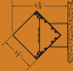
AS350-HO-DW AS350-MO-DW DIAMOND WALL MOUNT
