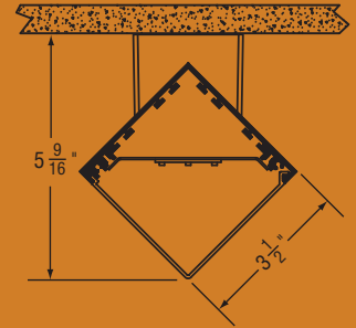
AS350-HO-DJ AS350-MO-DJ DIAMOND CEILING MOUNT
