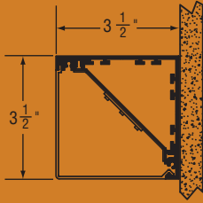
AS350-HO-FW AS350-MO-FW FLUSH WALL MOUNT (ADA COMPLIANT)
