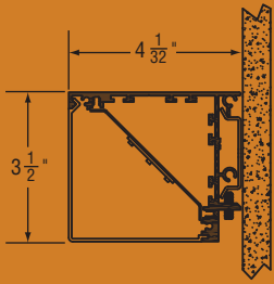
AS350-HO-W AS350-MO-W WALL MOUNT
