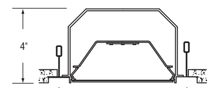
4" 6" "T" Centers MLR5-HO-TT MLR5-MO-TT Regular Tile
