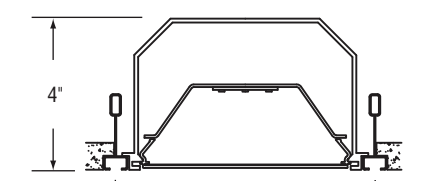
4" 6" "T" Centers MLR5-HO-SG MLR5-MO-SG Screw Slot Grid
