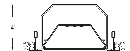
4" 6" "T" Centers MLR5-HO-FT MLR5-MO-FT Flush Tile
