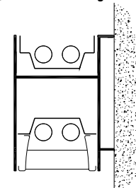
MLP3-I2/D2 T5 or T5HO Parabolic Baffle Shown
