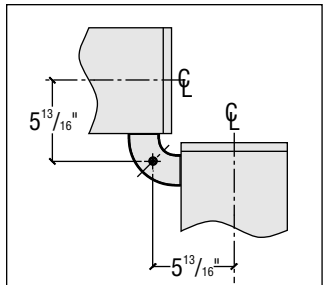
DCS - 90° CONNECTOR
