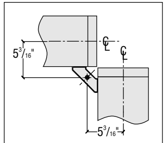
DRS - 90° CONNECTOR
